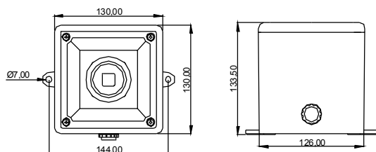
A105N Appello DC Dimensions.
