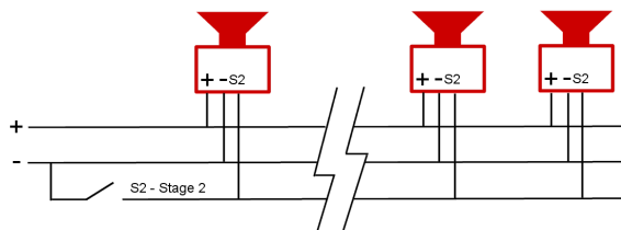
DC unit wiring configuration.
