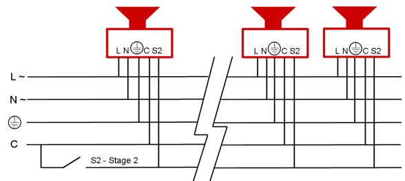
AC unit wiring configuration.
