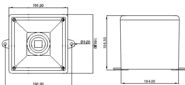
A112N Dimensions.
