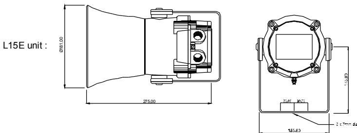
All dimensions are in millimetres.
