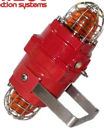
BExCBG05-05D Flameproof & Dust ignition proof beacons Zones 1, 2, 21 & 22 Ⓢ II 2G/D EEx d IIC T5 T100°C
