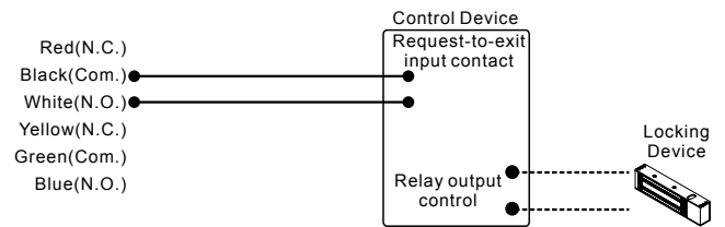
Fig A, The Locking Device was released by connecting the Control Device (as Keypad Proximity reader...etc.), PBA-840 switch output to 'Request-to-exit input contact' on control device.
