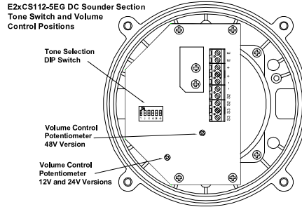
E2xCS112-5EG Sounder Section DC PCB Layout
