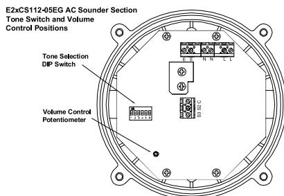
E2xCS112-5EG Sounder Section AC PCB Layout
