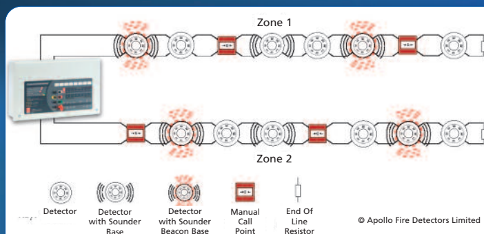
ALARMSENSE ZONE WIRING
